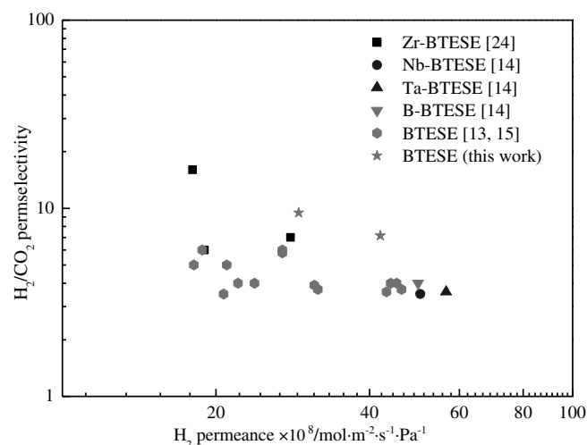
Fig. 10. Performance comparison of the organosilica membranes and other doped organosilica membranes.
