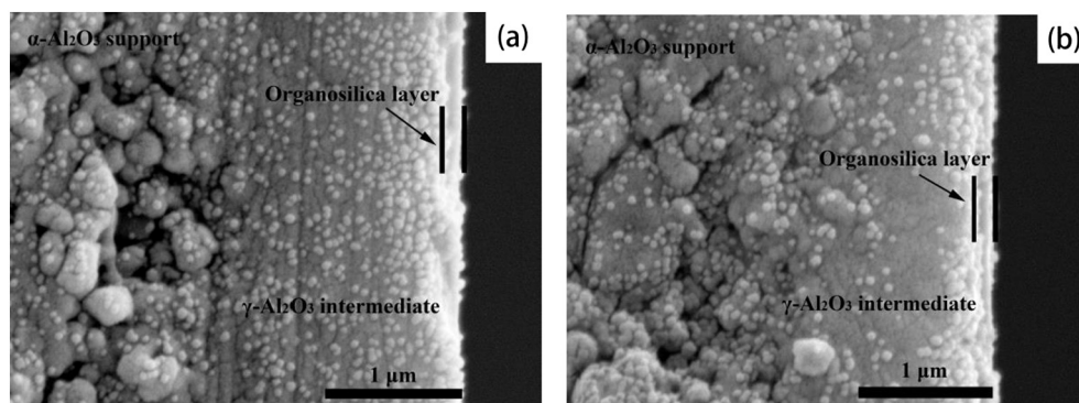
Fig. 8. Cross sectional SEM images of membranes (a) BTESE5 and (b) BTESE7.
