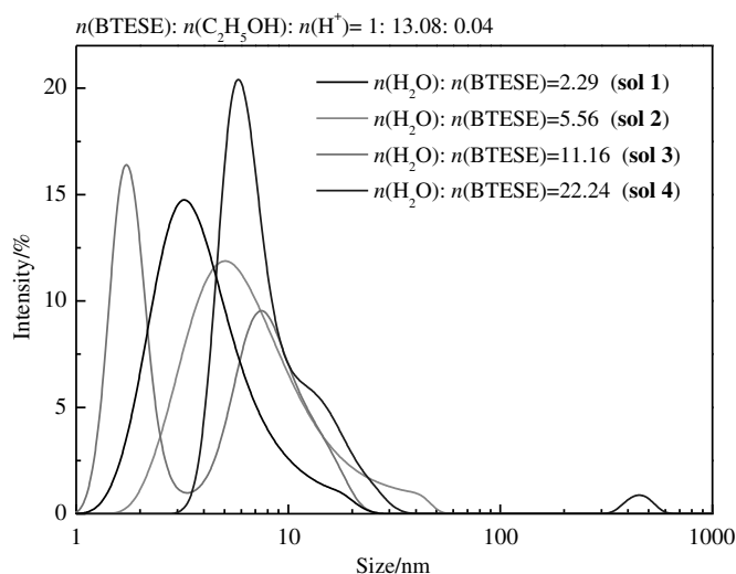
Fig. 1. Particle size distributions of the organosilica sols formed at different hydrolysis ratios.
