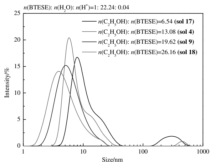
Fig. 3. Particle size distributions of the organosilica sols formed at different solvent ratios.
