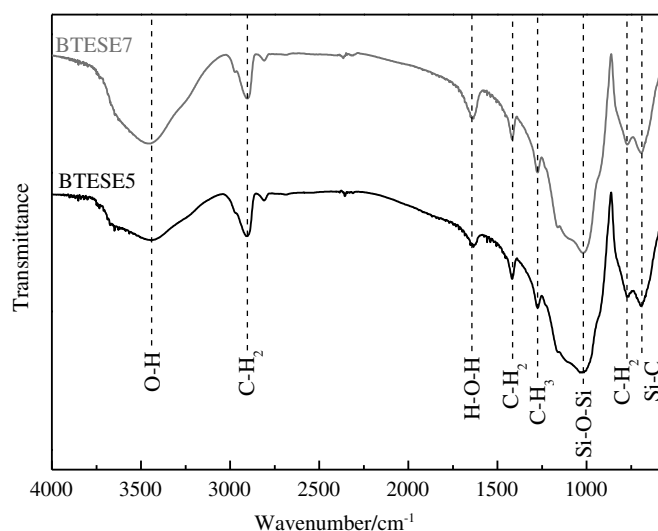
Fig. 5. FTIR spectra of the organosilica powders calcined at 400 °C under \text{N}_2 atmosphere.
