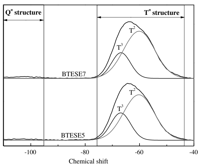
Fig. 6. Solid-state ^{29}\text{Si} MAS NMR spectra of the organosilica powders calcined at 400 °C under N 2 atmosphere.
