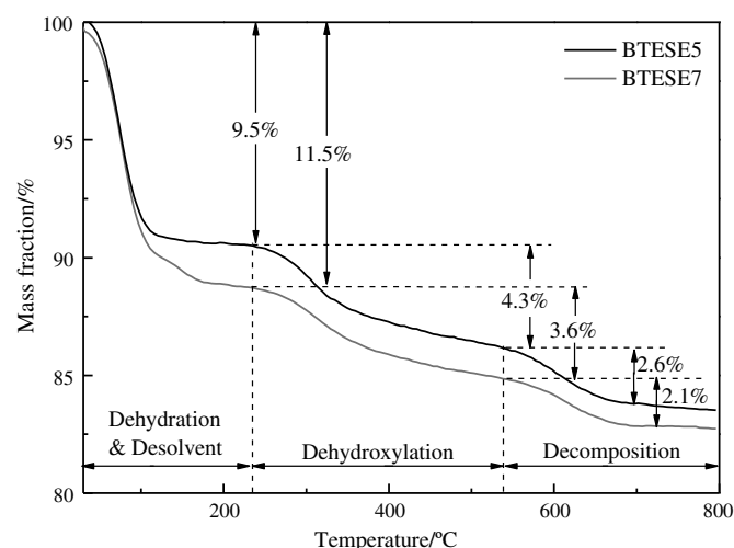
Fig. 4. Thermogravimetric curves of the organosilica gels.
