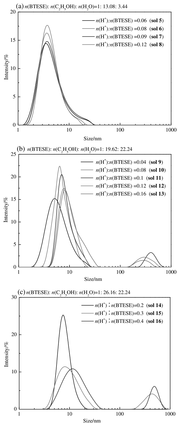
Fig. 2. Particle size distributions of the organosilica sols formed at different acid ratios.
