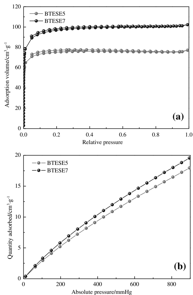
Fig. 7. N 2 adsorption–desorption (a) and CO 2 adsorption (b) isotherms of the organosilica powders calcined at 400 °C under N 2 atmosphere. 1 mmHg = 133.322 Pa.
