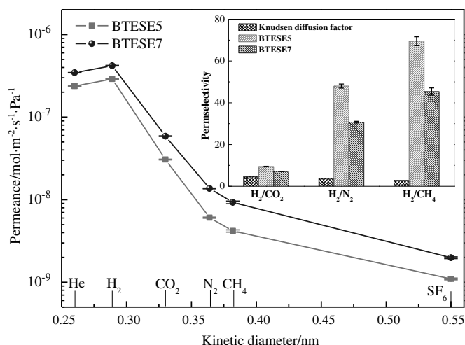
Fig. 9. Single gas permeances and permselectivities (inset) of the organosilica membranes calcined at 400 °C under N 2 atmosphere (measurement temperature 200 °C).
